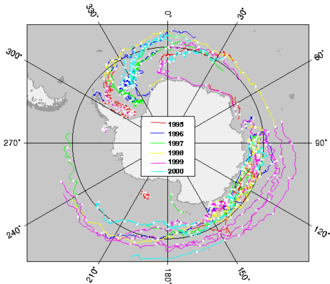
Figure 3. Typical Antarctic buoy tracks, 1995-2000. From the International Program for Antarctic Buoys, posted to the University of Tasmania web site at: http://www.antcrc.utas.edu.au/antcrc/special/buoys/buoys.html
