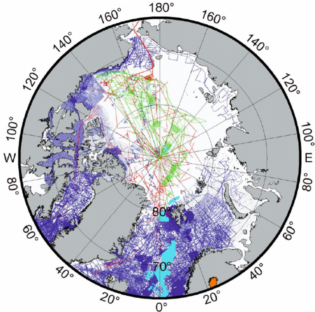
Figure 1. Depth sounding observation distribution for the Arctic Ocean. Red tracks are U.S. and U.K. submarine data; green are SCICEX data; blue are other sources including NGDC. Light blue is a multibeam survey area; orange is a grid model over the Gulf of Bothnia. (Prepared by M. Jakobsson, University of New Hampshire)
